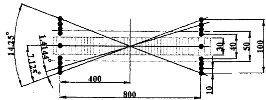
Fig. 8 Sensors location in the mobile robot
