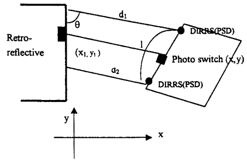
Fig. 19 Measured distances between PSD and retro-reflective object
