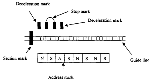
Fig. 3 Locations of a set of sensors
