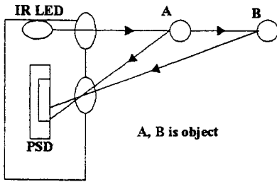
Fig. 13 Principle of PSD sensor
